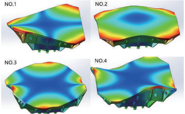
– Modal simulation diagram –
